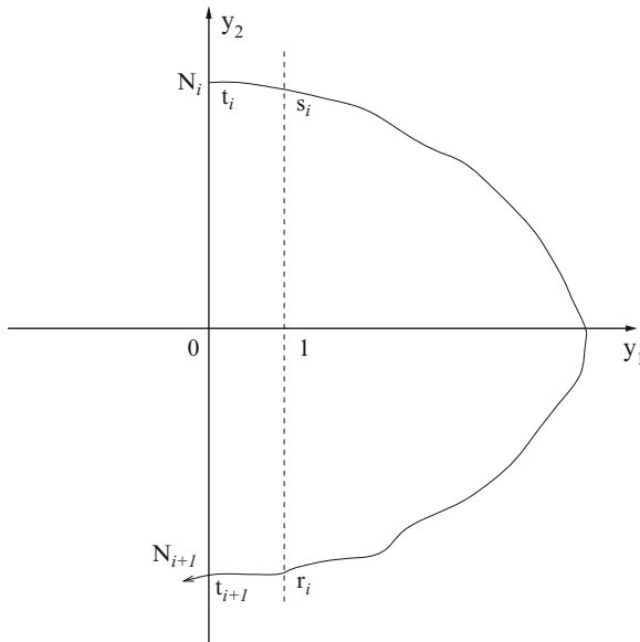
Figure 14.1: Proof of Lemma 14.5
