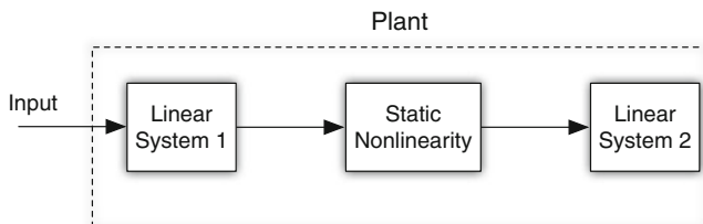
Figure 10.2: Static nonlinearity sandwiched between two linear systems
