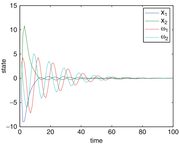
Figure 10.20: Semi-global stabilization via low-and-high-gain feedback with \alpha = 0.1
