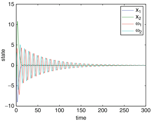
Figure 10.19: Semi-global stabilization via low-gain feedback
