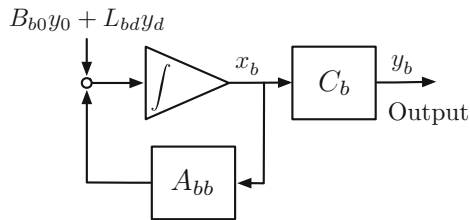
Figure 3.2: Non-right-invertible dynamics
